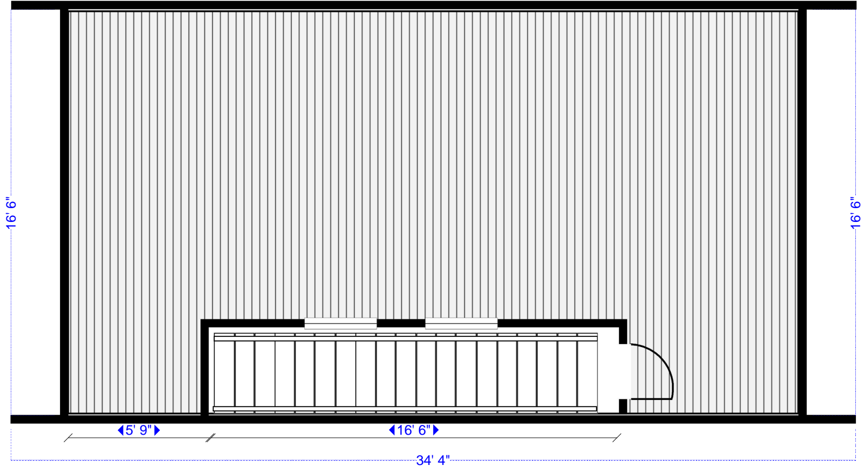
Level 3, Deck
